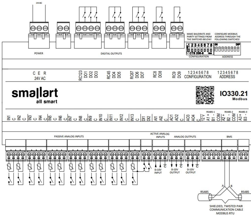
IO330.21 Connection Diagrams
