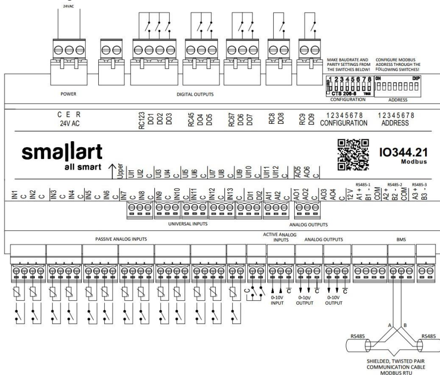
IO344.21 Connection Diagrams
