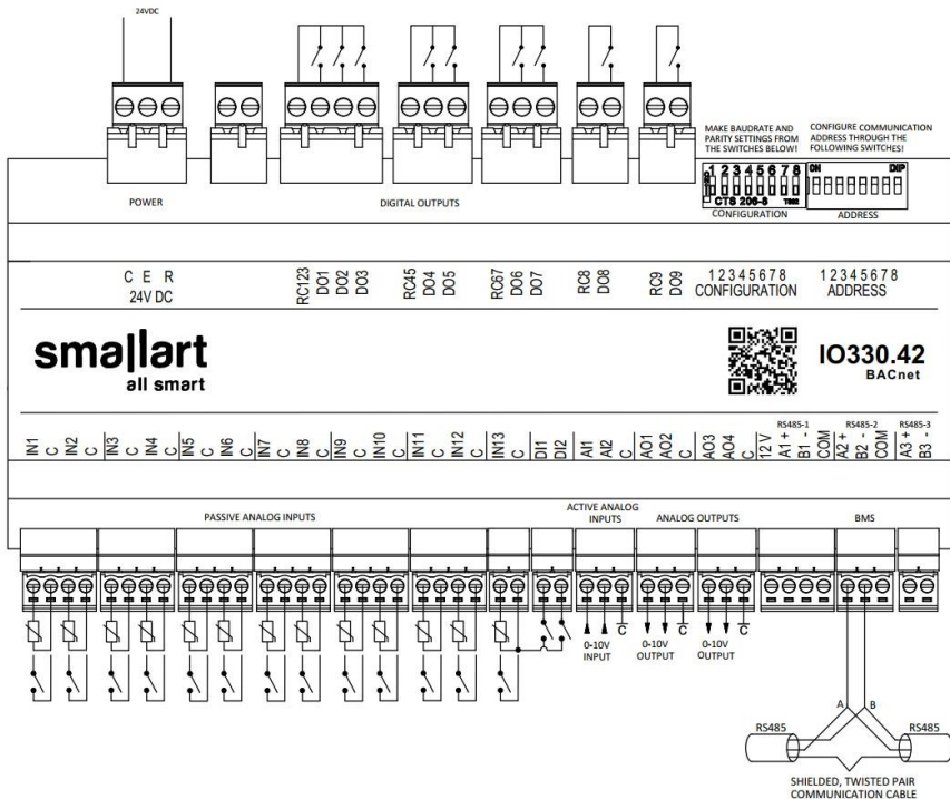
IO330.42 Connection Diagrams
