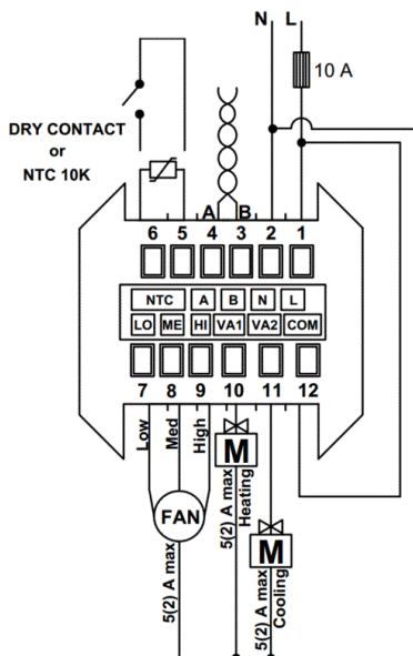
Connection Diagram for 4-Pipe Fan Coil
