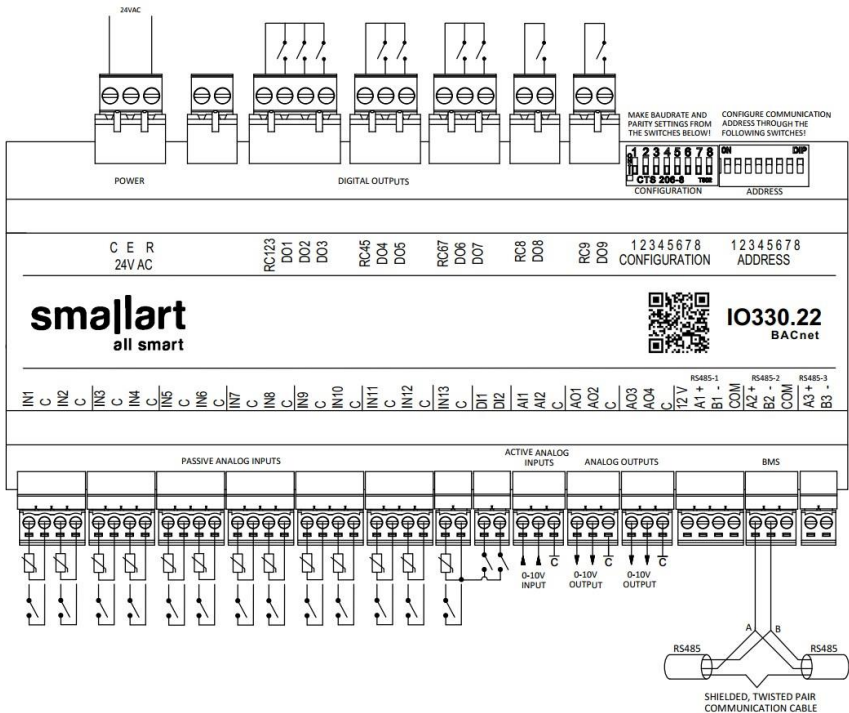
I0330.22 Connection Diagrams
