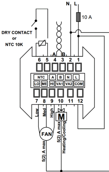
Connection Diagram for 2-Pipe Fan Coil
